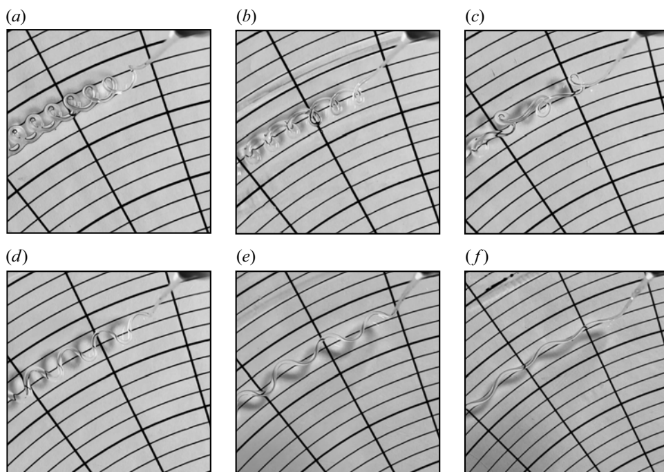
Figure 4. Selected experimental frames showing the patterns that recur in all cases dubbed the ‘main sequence’, for H = 5 cm, R = 15 cm and Q = 2 ml min ^{-1} : (a) outward and (b) inward loops occurring at low rotation rates \omega = 0.013 Hz and \omega = 0.019 Hz, respectively. Upon increasing \omega , the patterns transition to one-by-one (c) at \omega = 0.020 Hz, and then to meanders (d) at \omega = 0.025 Hz, which gradually flatten (e, f) to a catenary (not shown) at \omega = 0.060 Hz. In this case, the sharp shadows are caused by lighting from the side.
