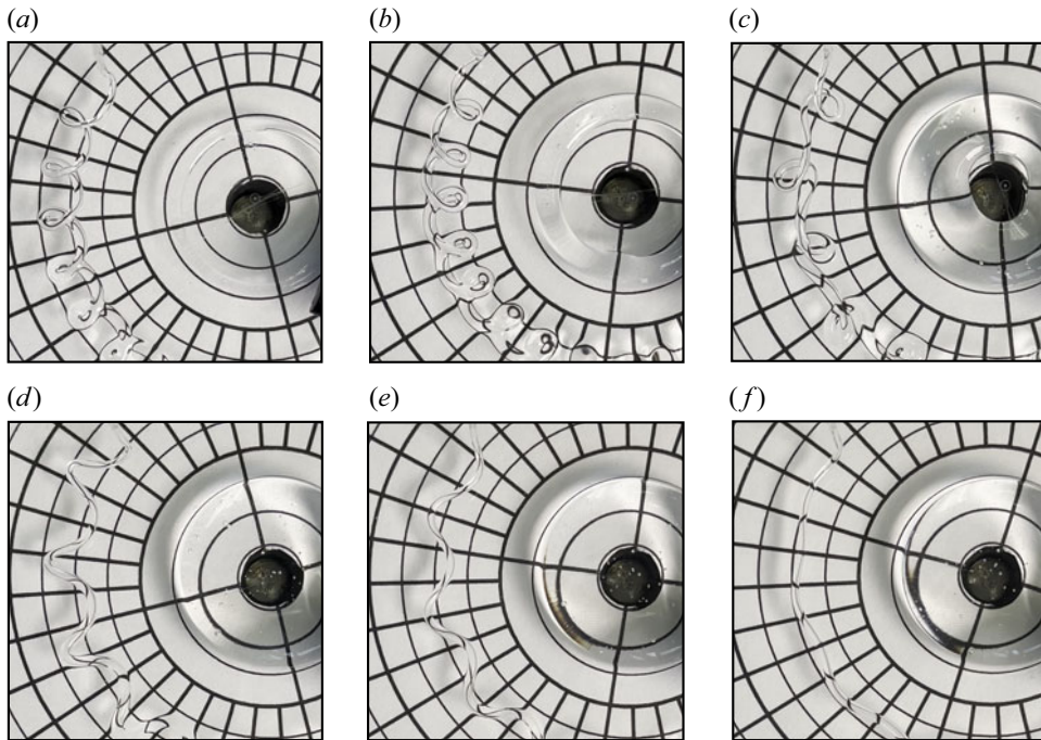
Figure 3. Selected experimental frames showing the patterns that recur in all cases dubbed the ‘main sequence’, for H = 5 cm, R = 3 cm and Q = 2 ml min ^{-1} : (a) outward and (b) inward loops occurring at the same, low rotation rate \omega = 0.079 Hz. Upon increasing \omega , the patterns transition to one-by-one (c) at \omega = 0.093 Hz, and then to meanders (d) at \omega = 0.13 Hz, which gradually flatten (e, f) to a circle (‘catenary state’, not shown) at \omega = 0.23 Hz.
