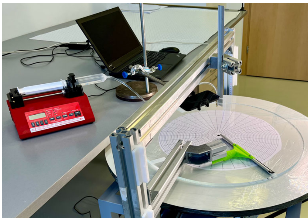
Figure 1. Experimental set-up. The rotating table supports an acrylic plate onto which the viscous thread falls, and its angular speed (anticlockwise) is controlled by a stepper motor connected to a laptop. Fluid is supplied at a constant flow rate using a (red) syringe pump visible on the left. Deposited oil is removed ahead of the point of contact of the stream with the plate by a (green) scraper, and removed from the centre between runs.
